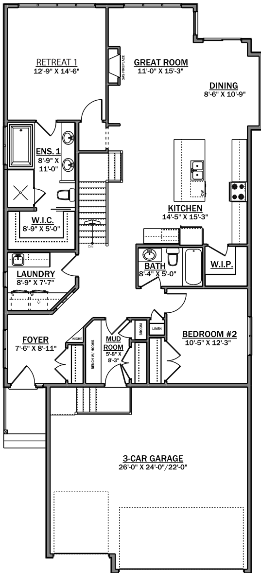
MAIN FLOOR PLAN 1568 SQ. FT.
