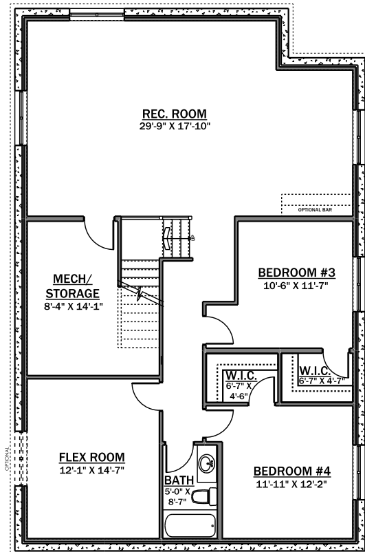
BASEMENT DEVELOPMENT 1174 SQ. FT.
