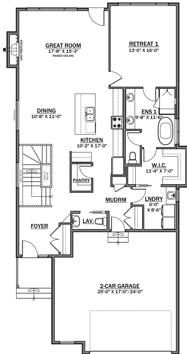
MAIN FLOOR PLAN 1493 SQ. FT.
