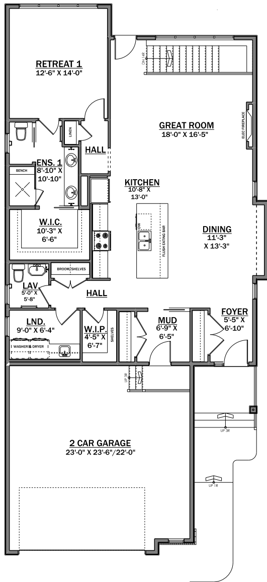
MAIN FLOOR PLAN 1413 SQ. FT.
