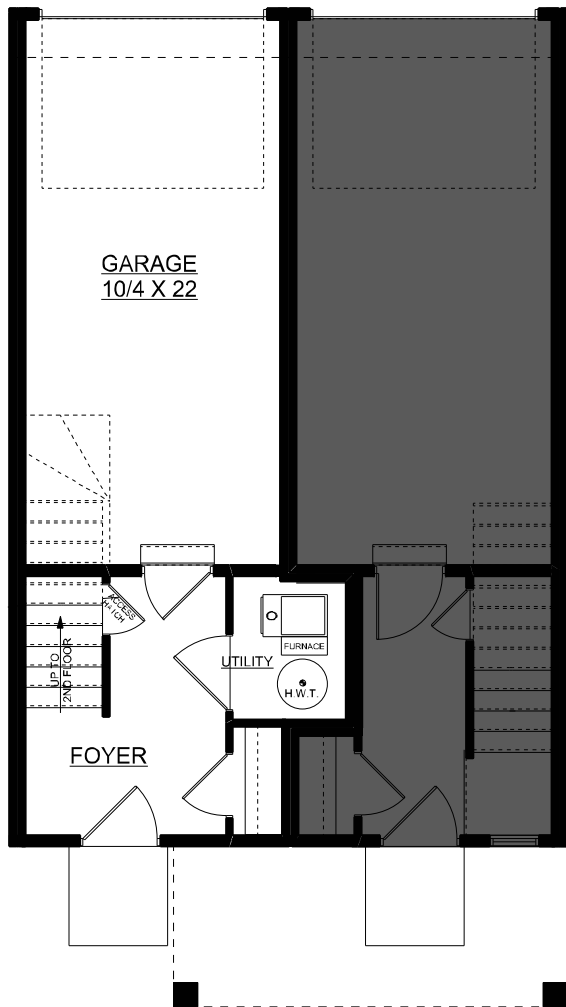
MAIN FLOOR PLAN 109 SQ. FT.
