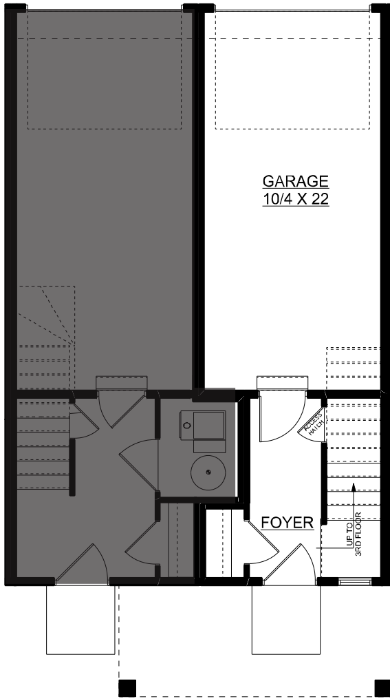
MAIN FLOOR PLAN 117 SQ. FT.
