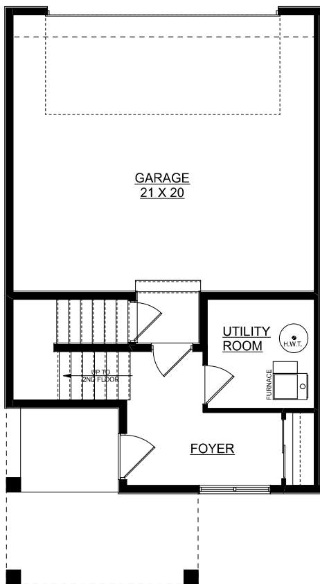
MAIN FLOOR PLAN 178 SQ. FT.
