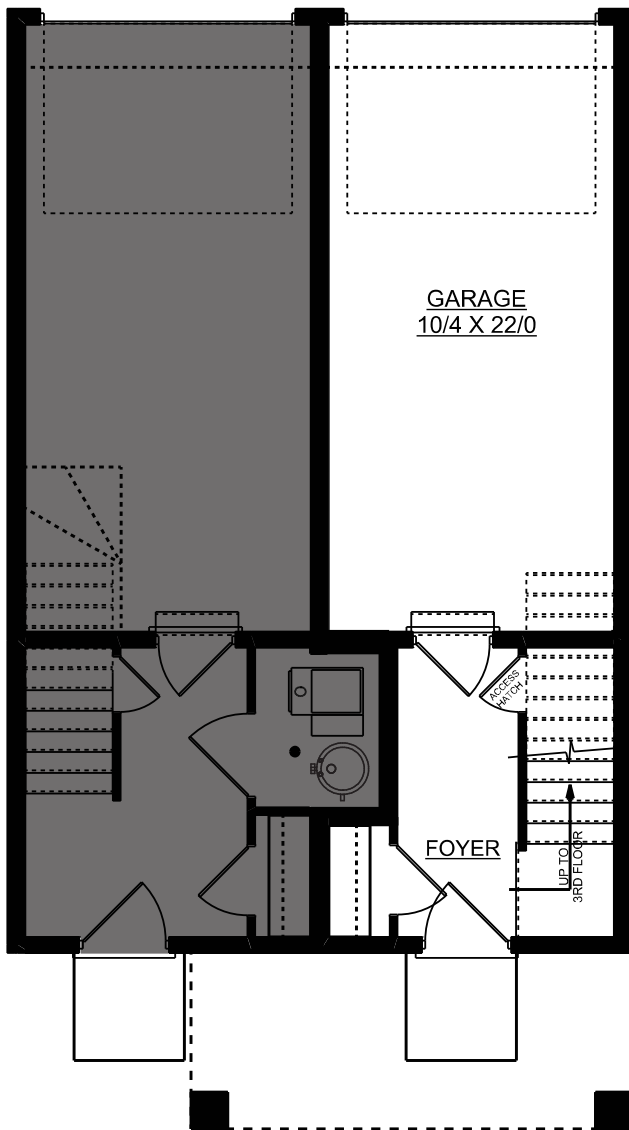
MAIN FLOOR PLAN 117 SQ. FT.
