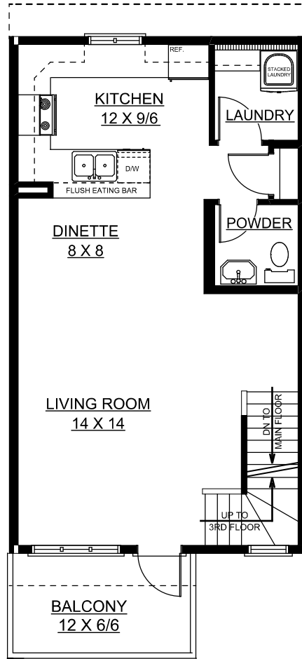
SECOND FLOOR PLAN 576 SQ. FT.
