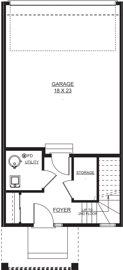
MAIN FLOOR PLAN 166 SQ. FT.
