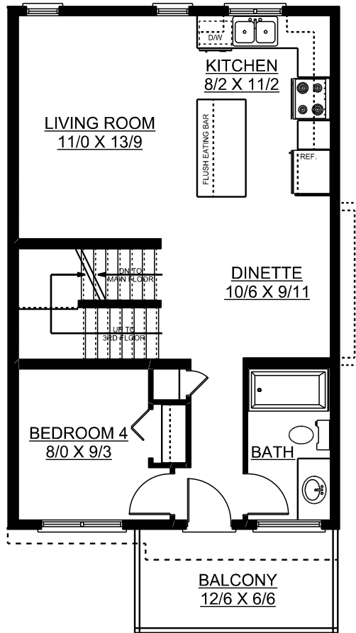
SECOND FLOOR PLAN 578 SQ.FT.
