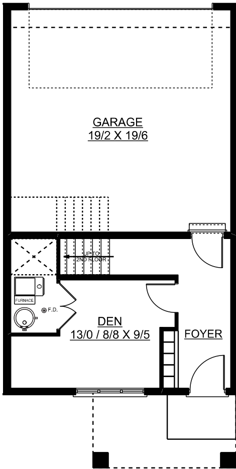
MAIN FLOOR PLAN 280 SQ.FT.
